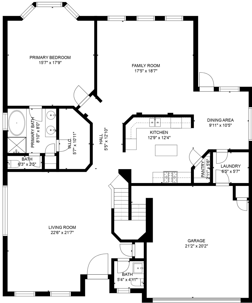
FLOOR 1
